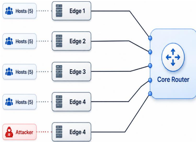
Figure 2. Network testbed topology. The central core router is connected to four edge routers, each with 5 end hosts. Attacker node connected to the core
